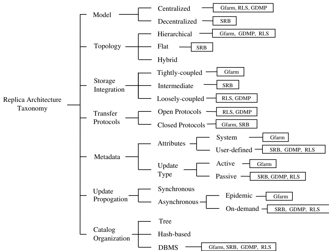
Figure 14: Mapping of Data Replication Architecture Taxonomy to Various Systems.
