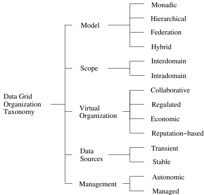
Figure 4: Data Grid Organization Taxonomy.
