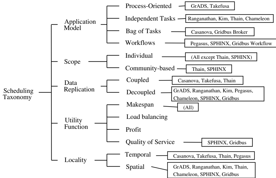
Figure 16: Mapping of Resource Allocation and Scheduling Taxonomy to Various Systems.
