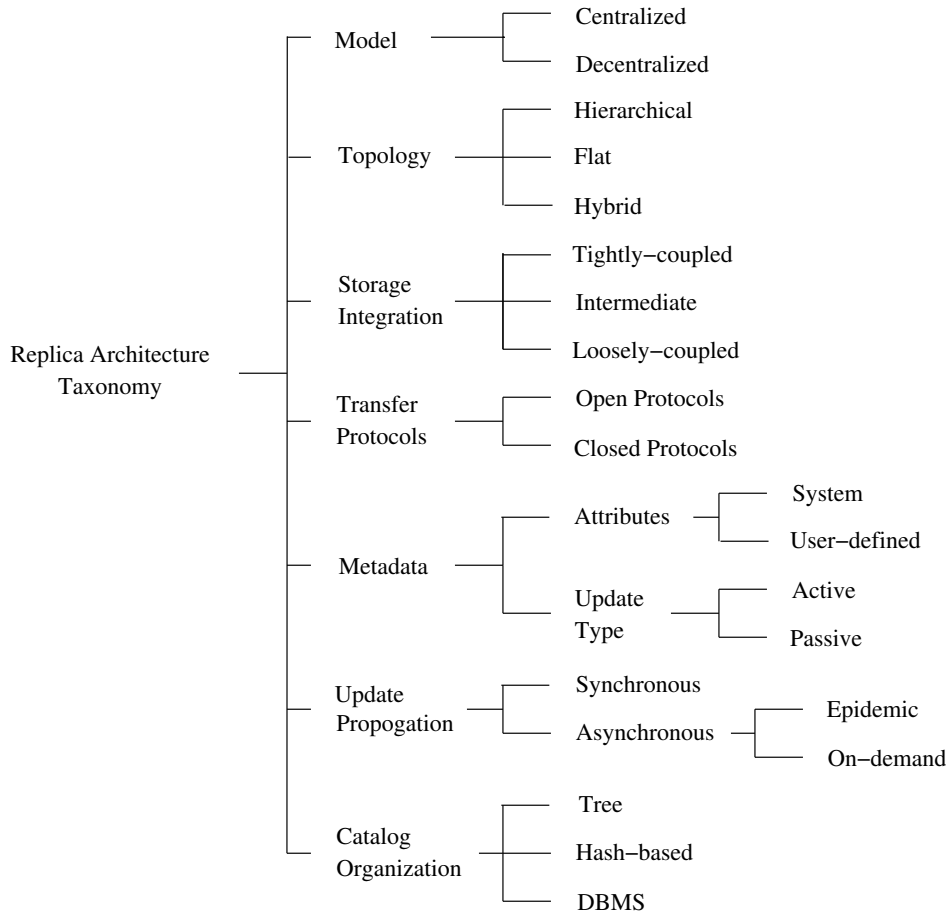
Figure 9: Replica Architecture Taxonomy.
