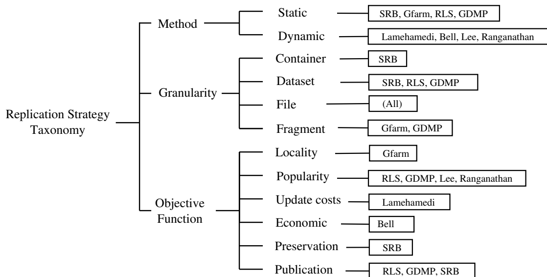
Figure 15: Mapping of Data Replication Strategy Taxonomy to Various Systems.
