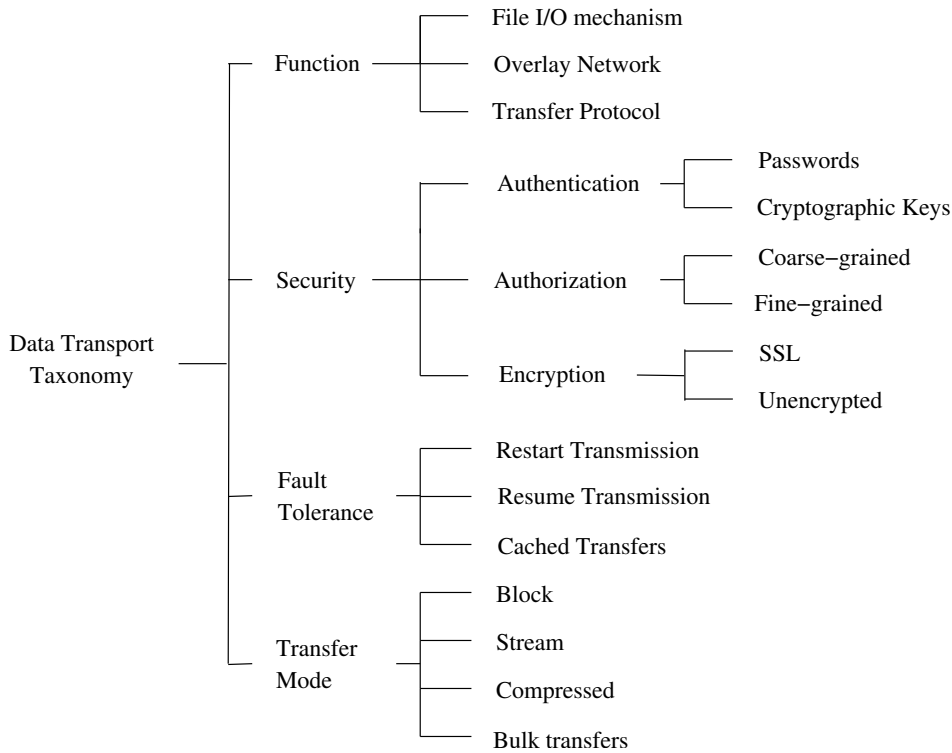
Figure 6: Data Transport Taxonomy.
