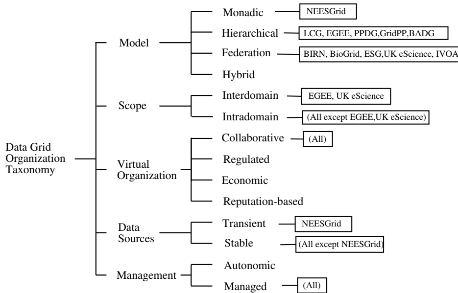
Figure 12: Mapping of Data Grid Organization Taxonomy to Data Grid Projects.
