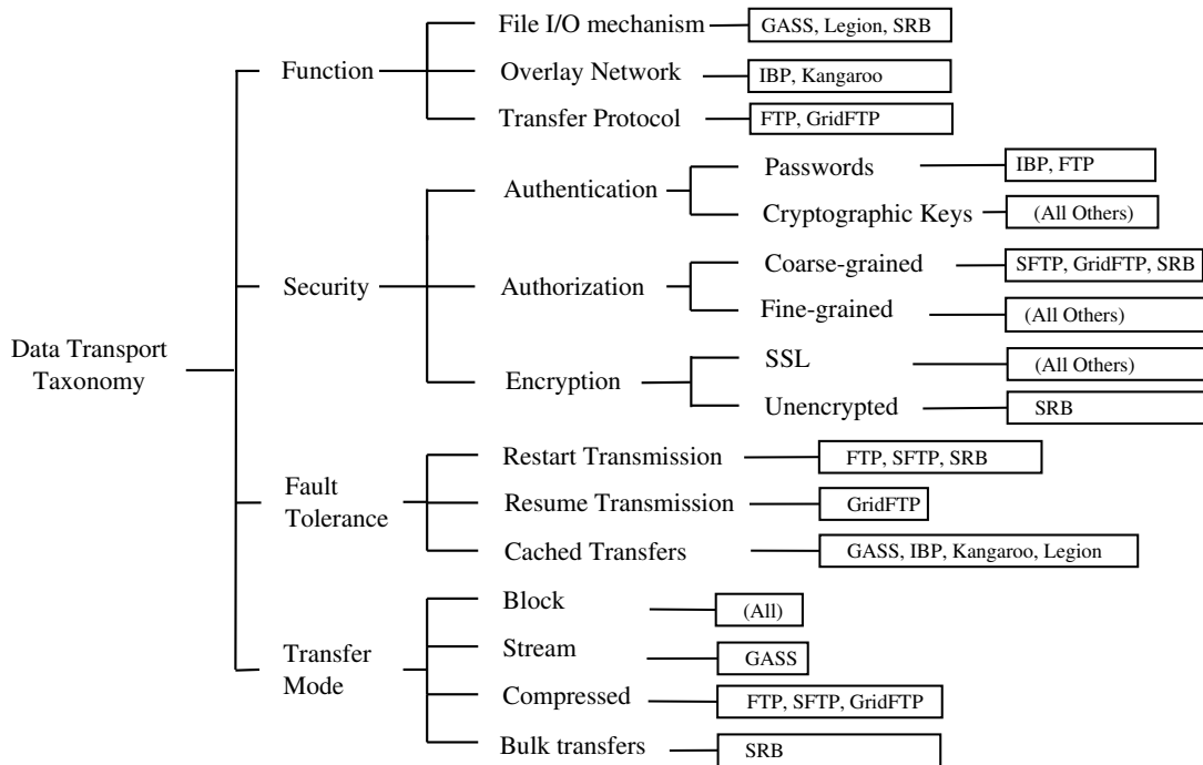
Figure 13: Mapping of Data Transport Taxonomy to Various Projects.
