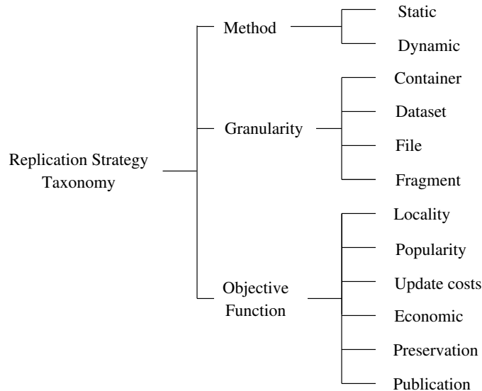
Figure 10: Replication Strategy Taxonomy.
